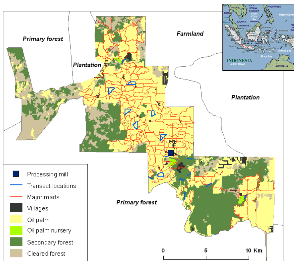
Figure 1. Distribution of habitat types within the case study concession showing existing roads and the location of ecological survey transects.
