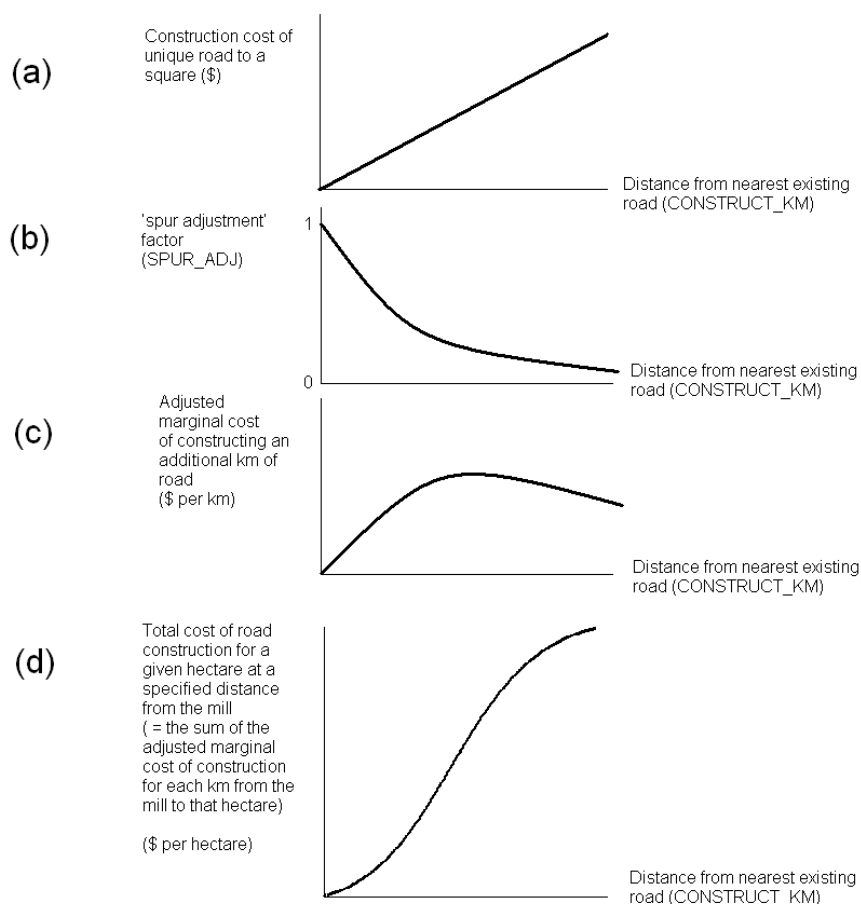
Figure3: Sketch of relationships adjusting for spurring effects in road construction costs.
