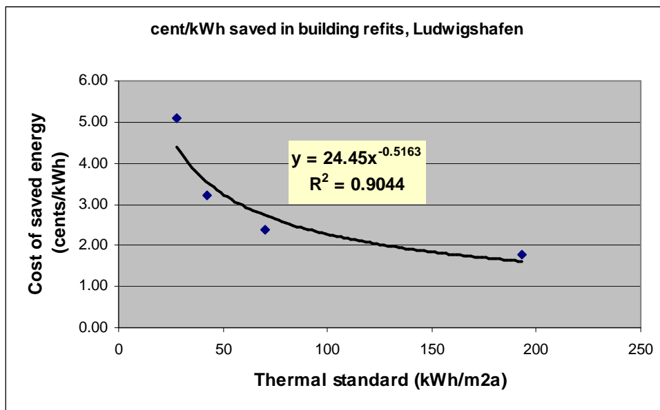
Fig 1. Costs of energy saved over the lifetime of renovations in the Ludwigshafen study. Data source: Enseling and Hinz (2006).
