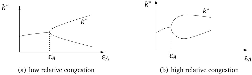
Figure 2: Bifurcation diagram.
