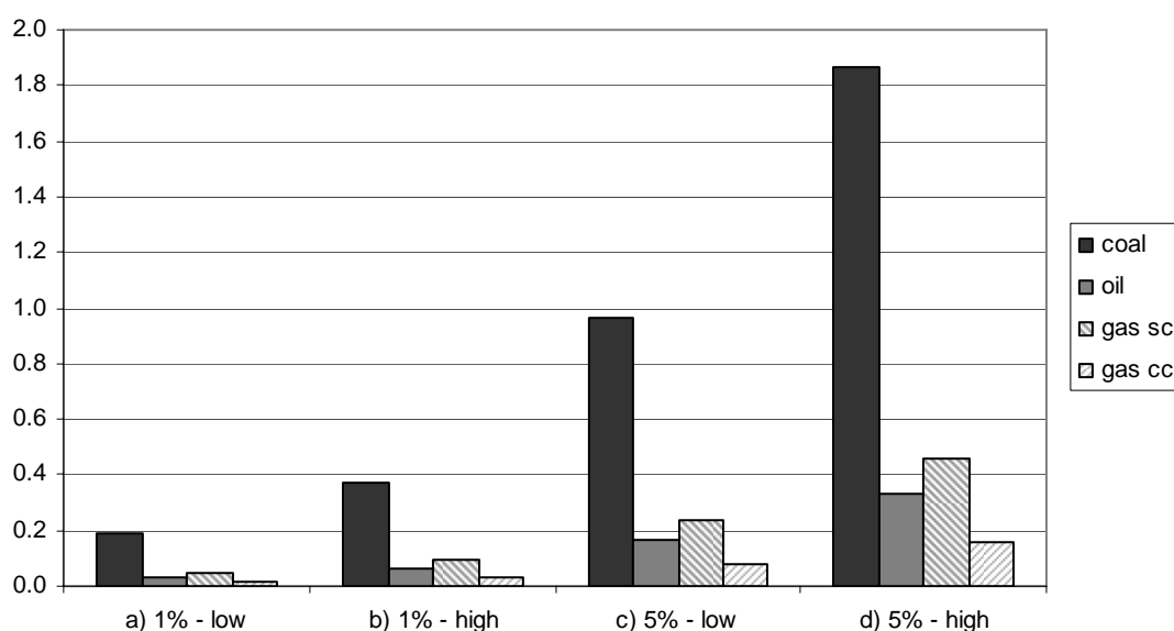
Figure 9: Four scenarios for the emission reduction potential of R&M in Brazil from 2005-2020 (Mt CO 2 e)
