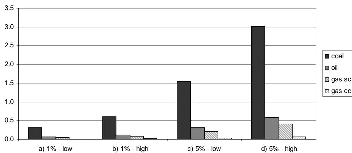
Figure 14: Four scenarios for the emission reduction potential of R&M in Indonesia from 2005-2020 (Mt CO 2 e)
