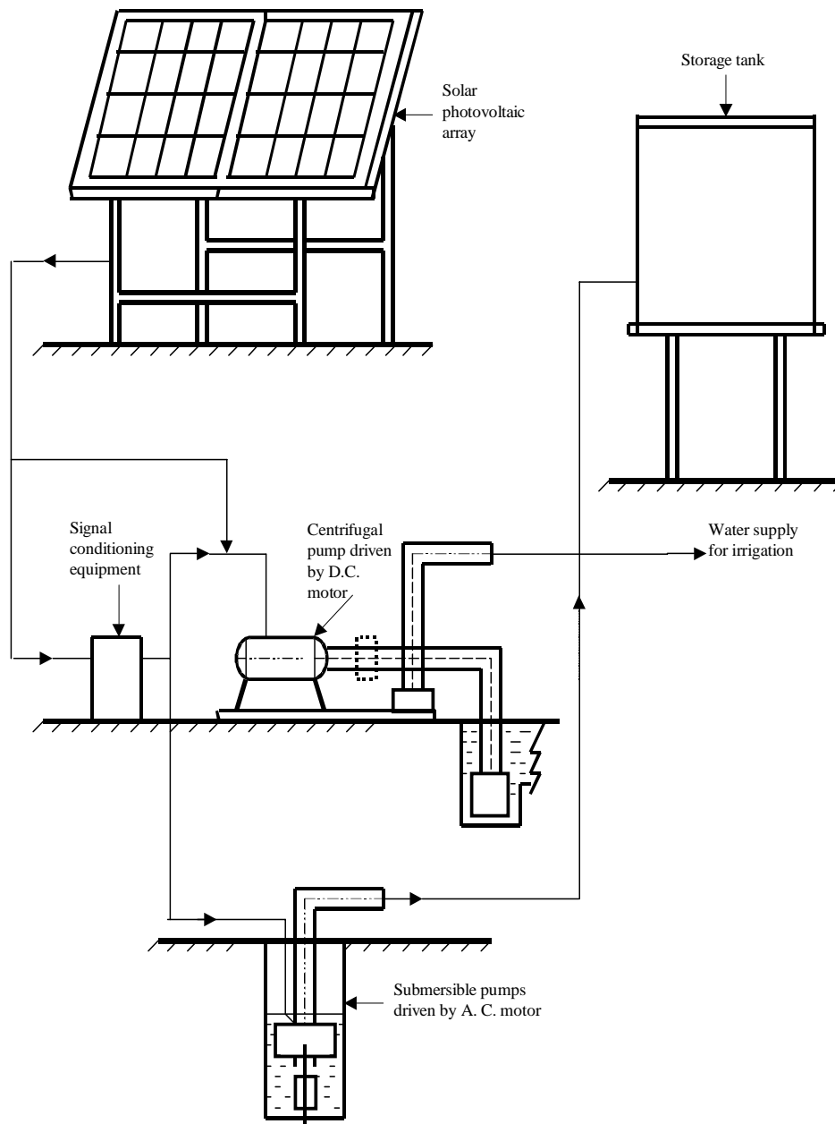
Figure 2. Schematic diagram of solar photovoltaic water pump
