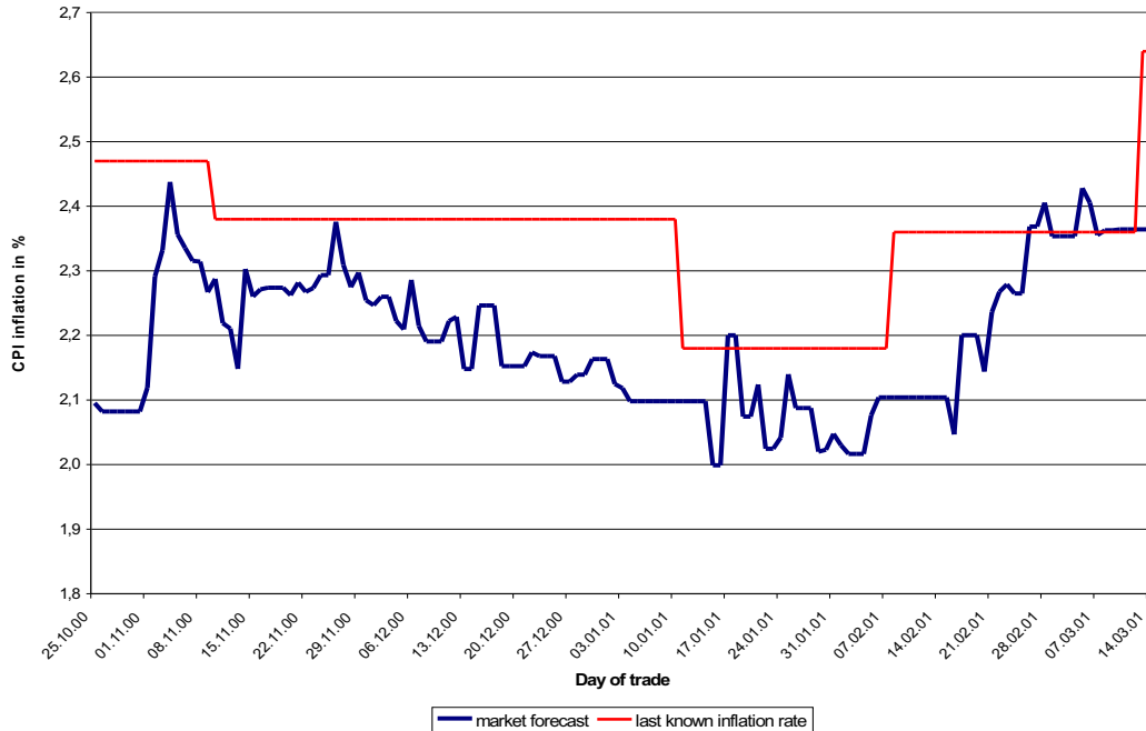
Figure 5: Mean inflation forecast for February 2001 and last known inflation rate
