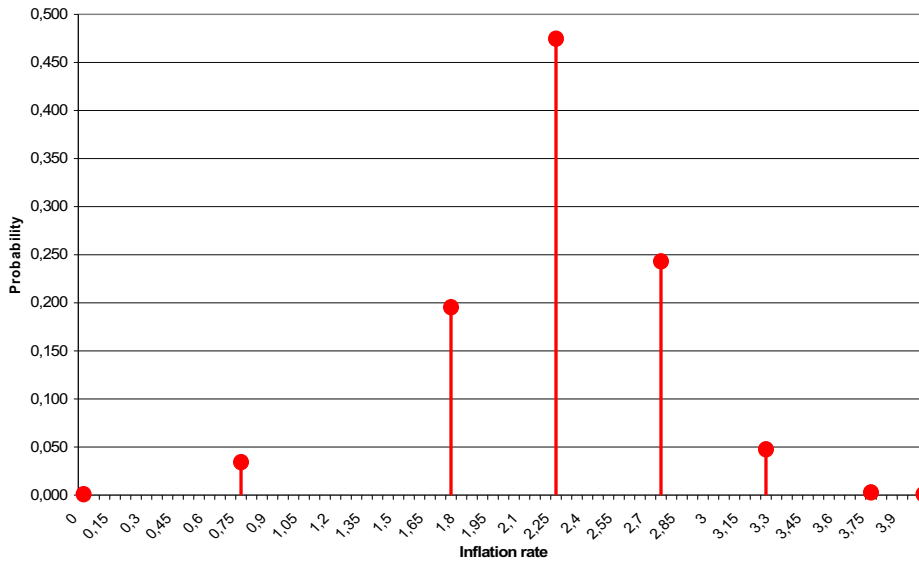
Figure 9: Distribution of inflation forecast on 12th December 2000
