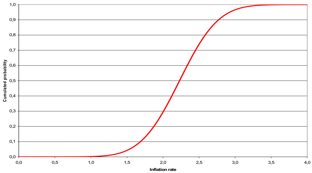
Figure 10: Cumulative probability function of the market inflation forecast on 12th December 2000
