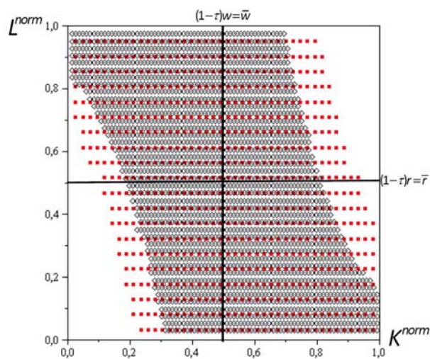
Figure 5: Overlap in response to q (smaller, grey shaded area: q = 0.45 ; larger, red shaded area:
