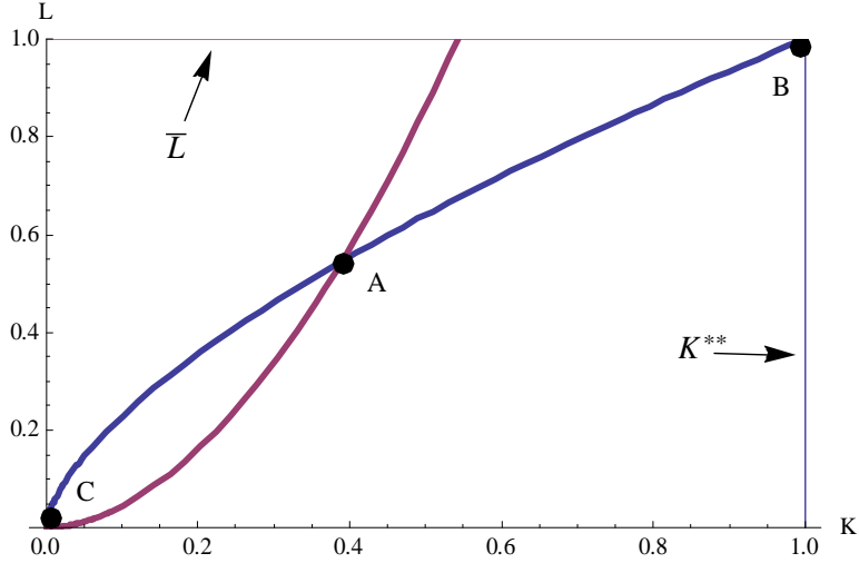
Figure 3: Multiple equilibria.
