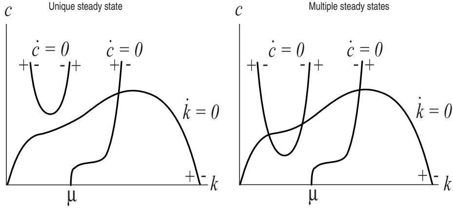
Figure 3: The phase diagrams of the model.
