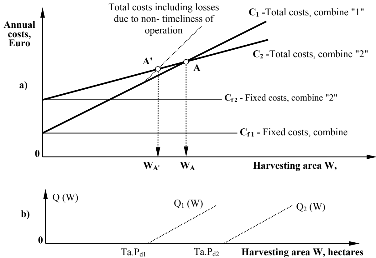
Figure 2: Model for estimating the break-even harvesting area for combines of different size
