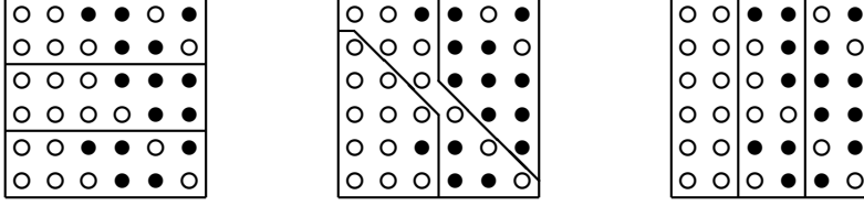
Figure 2: Unlinked districtings
