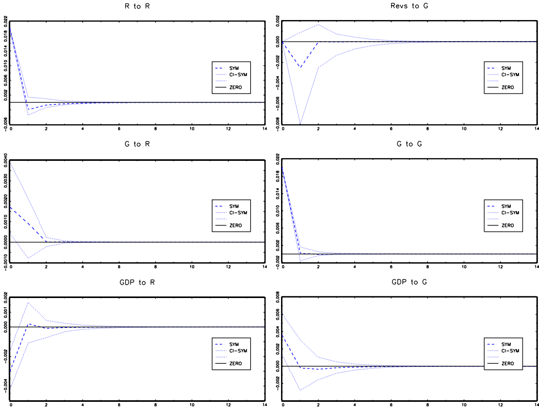
Figure 5: Linear Impulse Responses, Shocks in R and G
