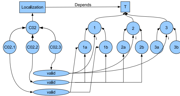
Figure 2: Ontology containing concepts Localization and T with individuals
