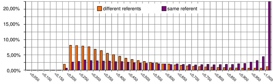
Figure 4: Probability distributions generated by the learned document pair classifier \delta , based on the optimized combination of the retrieval models \mathcal{R}_1, \dots, \mathcal{R}_5 .
