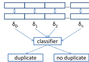
Figure 3: A duplicate detection algorithm using a classification algorithm. In the learning phase, the algorithm’s inputs are the distances between the correspondent attributes and the knowledge about whether or not the instances are duplicates, in the application phase that knowledge is deduced through the classifier that is the learning phase’s output.
