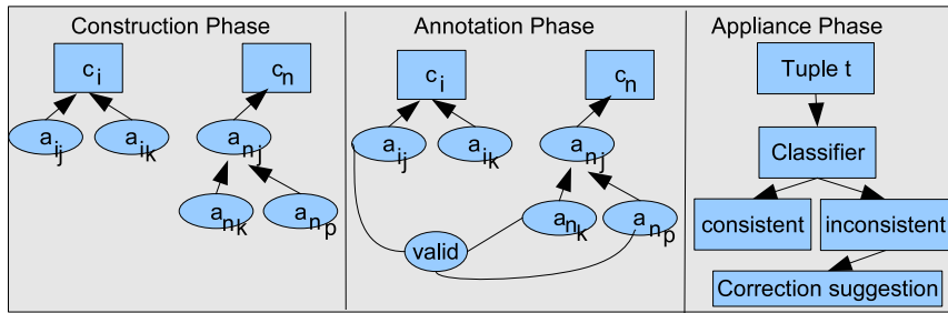
Figure 1: Overview of an inconsistency detection algorithm using a domain ontology
