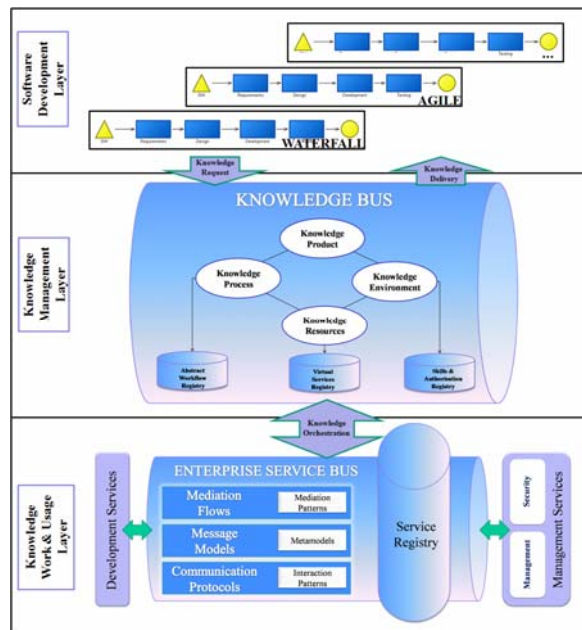
Figure 2: The Knowledge Bus Approach
