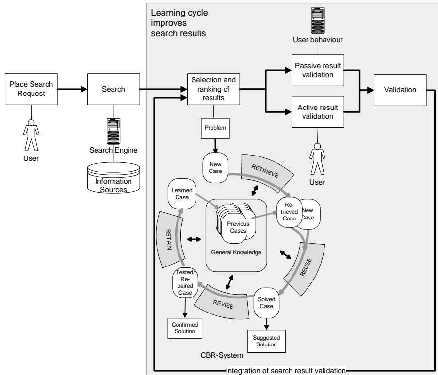
Figure 2: Process of self-learning search engine.
