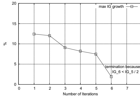
Figure 3: Convergence of the maximum IG growth
