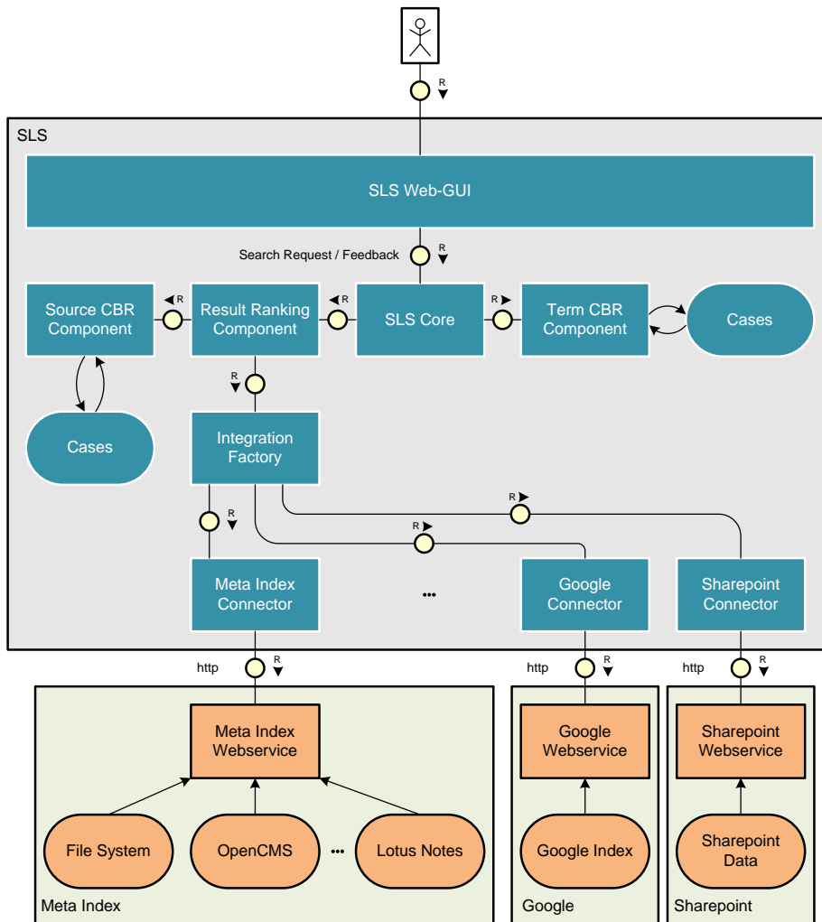
Figure 1: SLS prototype architecture
