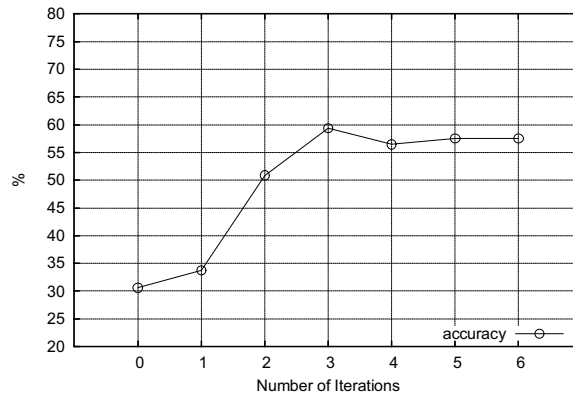
Figure 4: Boosted Accuracy
