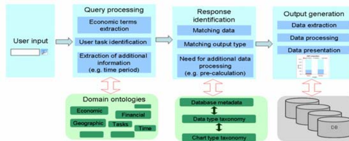
Figure 3: System framework
