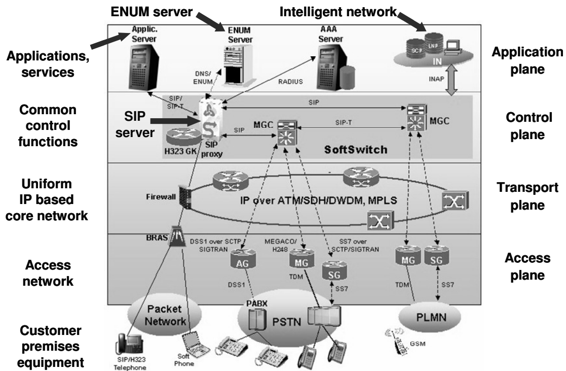
Figure 6: NGN reference architecture and addressing solutions
