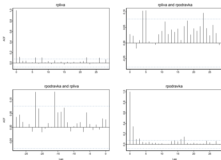
Figure 2: Correlograms and cross-correlograms between Pliva and Podravka square returns
