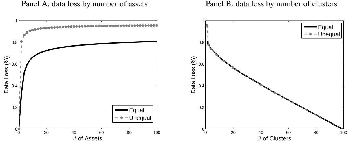
Figure 2: Illustration of the data loss implied by the refresh time sampling scheme
