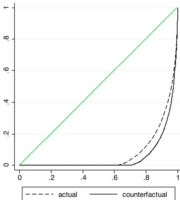
Figure 2 Lorenz-curve for the distribution of the R&D personnel (Germany)
