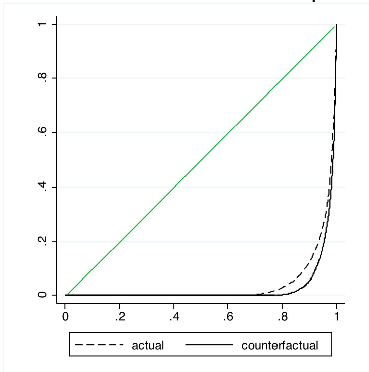
Figure 1 Lorenz-curve for the distribution of the R&D personnel (Finland)
