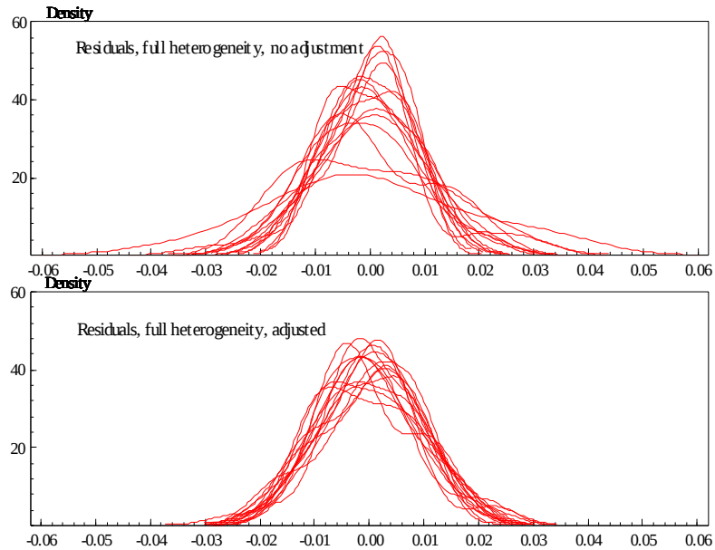
Figure 4: Density Distribution of the Residuals before (Top) and after (Bottom) Correcting for Heteroskedasticity
