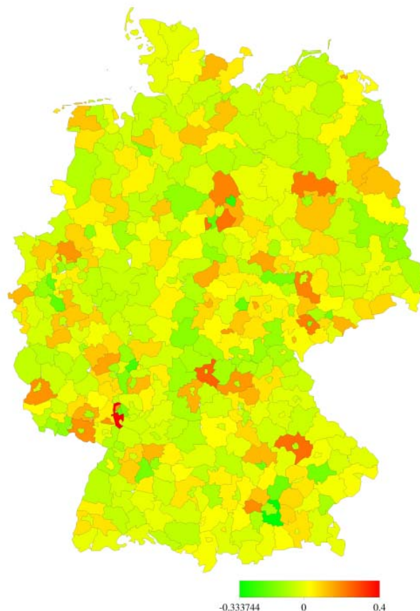
FIGURE 5: Efficiency of German NUTS 3 regions, non-spatial structural factor f_{rand(i)} , 2004
