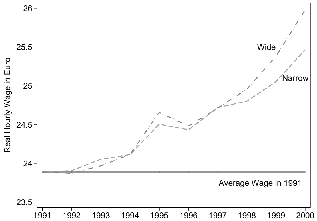
Figure 6: Cumulated marginal effects of outsourcing for workers with high skill requirements
