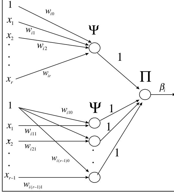
Figure 4.3: Hybrid node h_i(x) with r input variables
