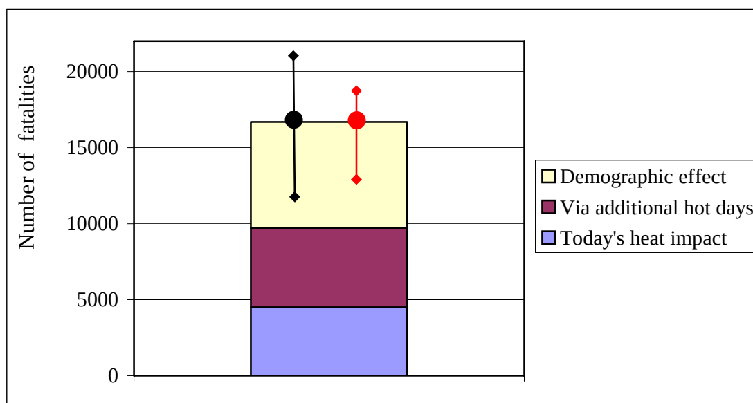
Figure 4: Number of heat induced deaths p. a. in Germany, 2071-2100 (exponential extrapolation for extreme heat stress)
