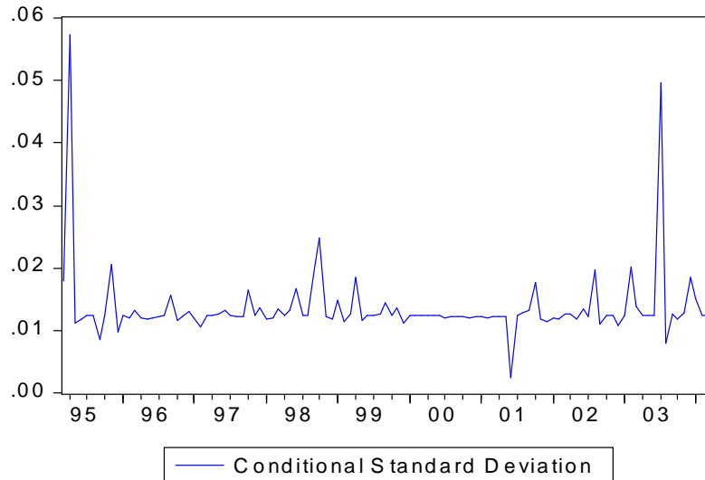
Figure 3: TARCH Conditional SD for Hungary
