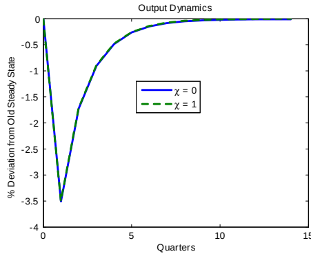
Figure 2: Output response after a disinflation from 4% to 0
