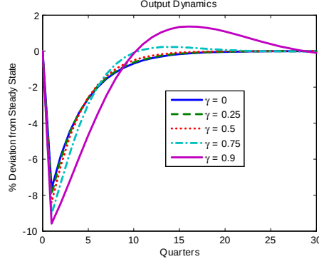
Figure 6: Decreasing returns to scale to labor and the effect of real rigidities
