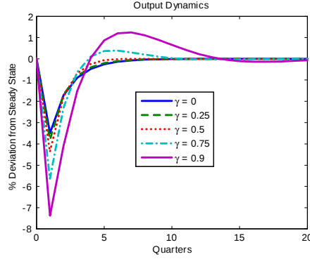
Figure 4: The effect of real rigidities on the output response to a disinflation
