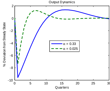
Figure 7: DRTS and output response after a disinflation from 4% to 0 ( \gamma = 0.9 )
