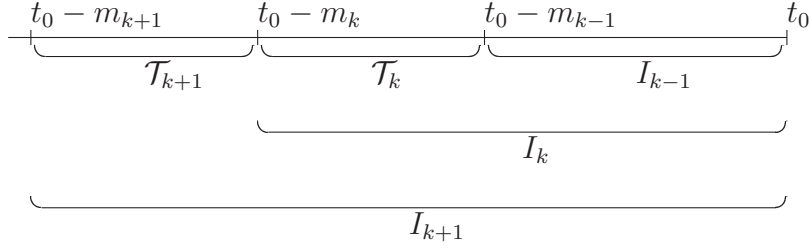
Figure 2: Interval Selection
