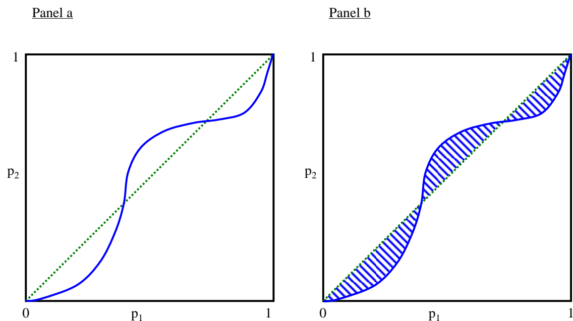
Figure 2 Theoretical PP-plot (panel a) and the associated HM-index (panel b)
