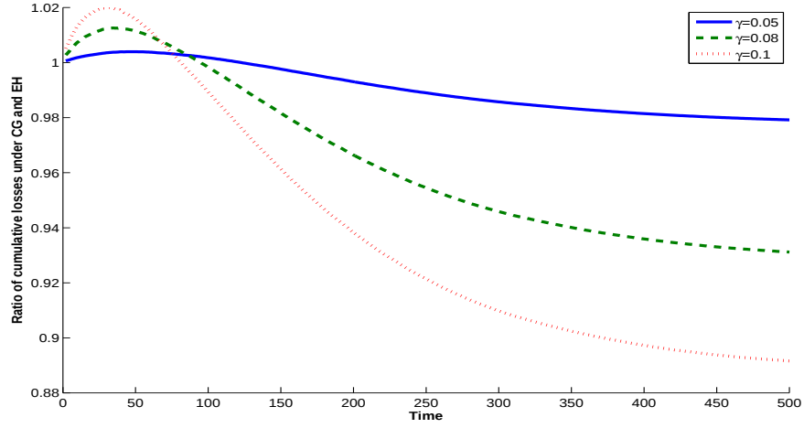
Figure 4: The dynamics of welfare losses (ratio of cumulative consumption equivalents under CG and EH) under constant gain learning, with initial beliefs at the rational equilibrium
