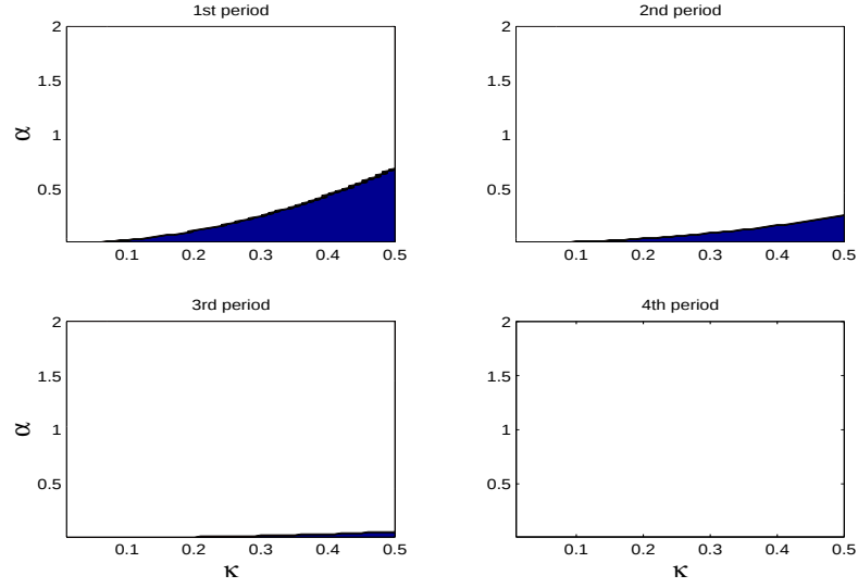
Figure 6: Values of \alpha and \kappa for which \delta_{\pi}^{dg} is increasing in the first four periods. From the fourth period on \delta_{\pi}^{dg} is always decreasing. ( \beta = 0.99 )
