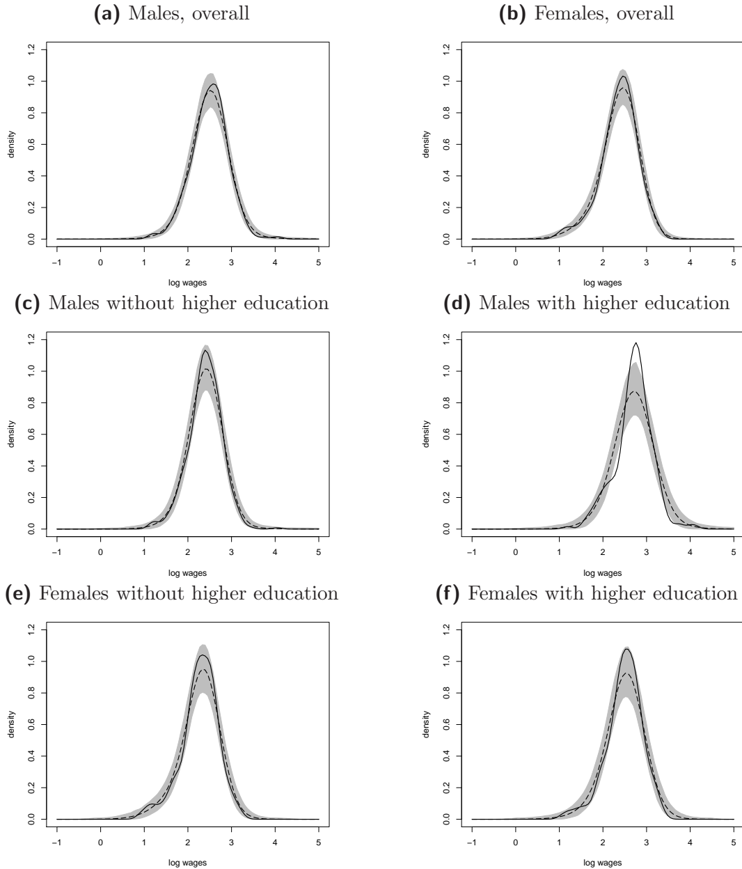
Figure 1: Goodness-of-fit check for wages: posterior predictive (dashed) vs. actual distribution (solid) for the model estimated by conditioning labor market outcomes on education (panels 1c, 1d, 1e and 1f) and without conditioning on education (panels 1a and 1b).
