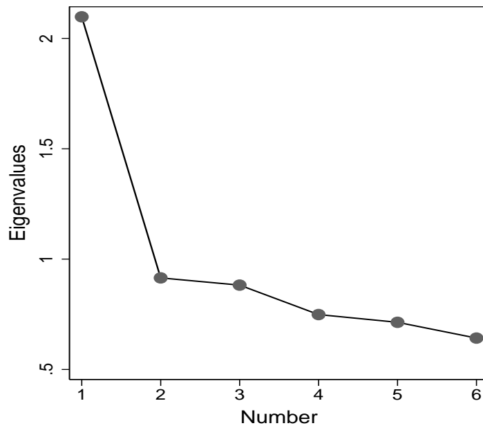
Figure A.2: Scree plot: locus of control measurements (6 items with high loadings only, reflecting an external locus of control: Q2, Q3, Q4, Q6, Q7 and Q9)
