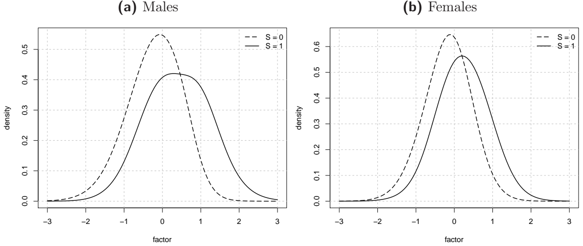
Figure 2: Latent factor distribution by levels of education: people with higher education ( S = 1 ) and without higher education ( S = 0 ).
