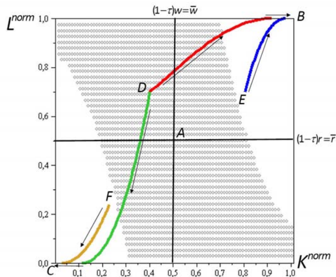
Figure 4: Three steady states and four possible equilibrium trajectories.
