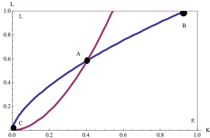
Figure 3: Multiple equilibria.
