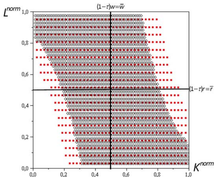
Figure 5: The size of the overlap in response to changes in q .
