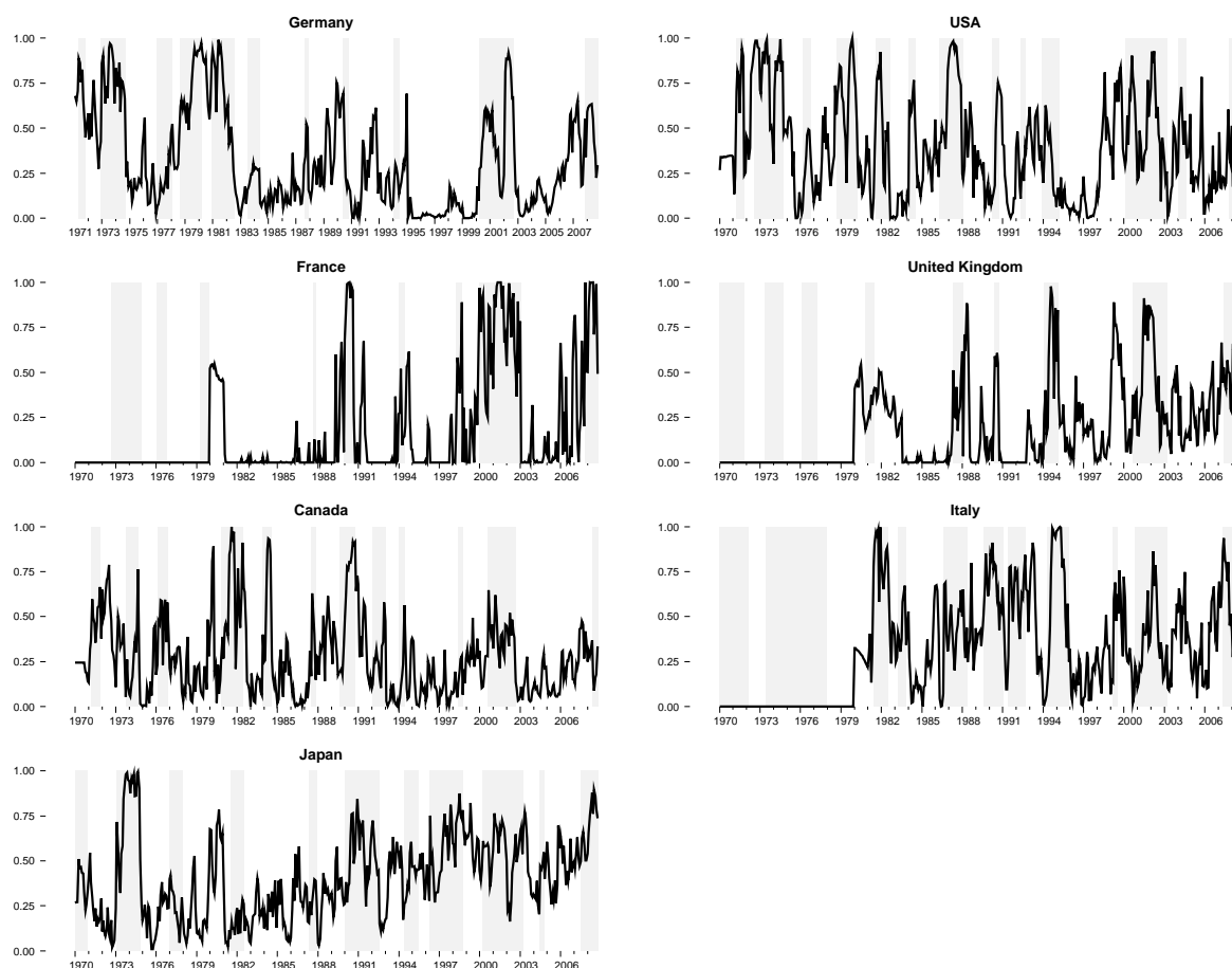
Figure 3: In-sample recession probabilities - all variables - 1 lag
