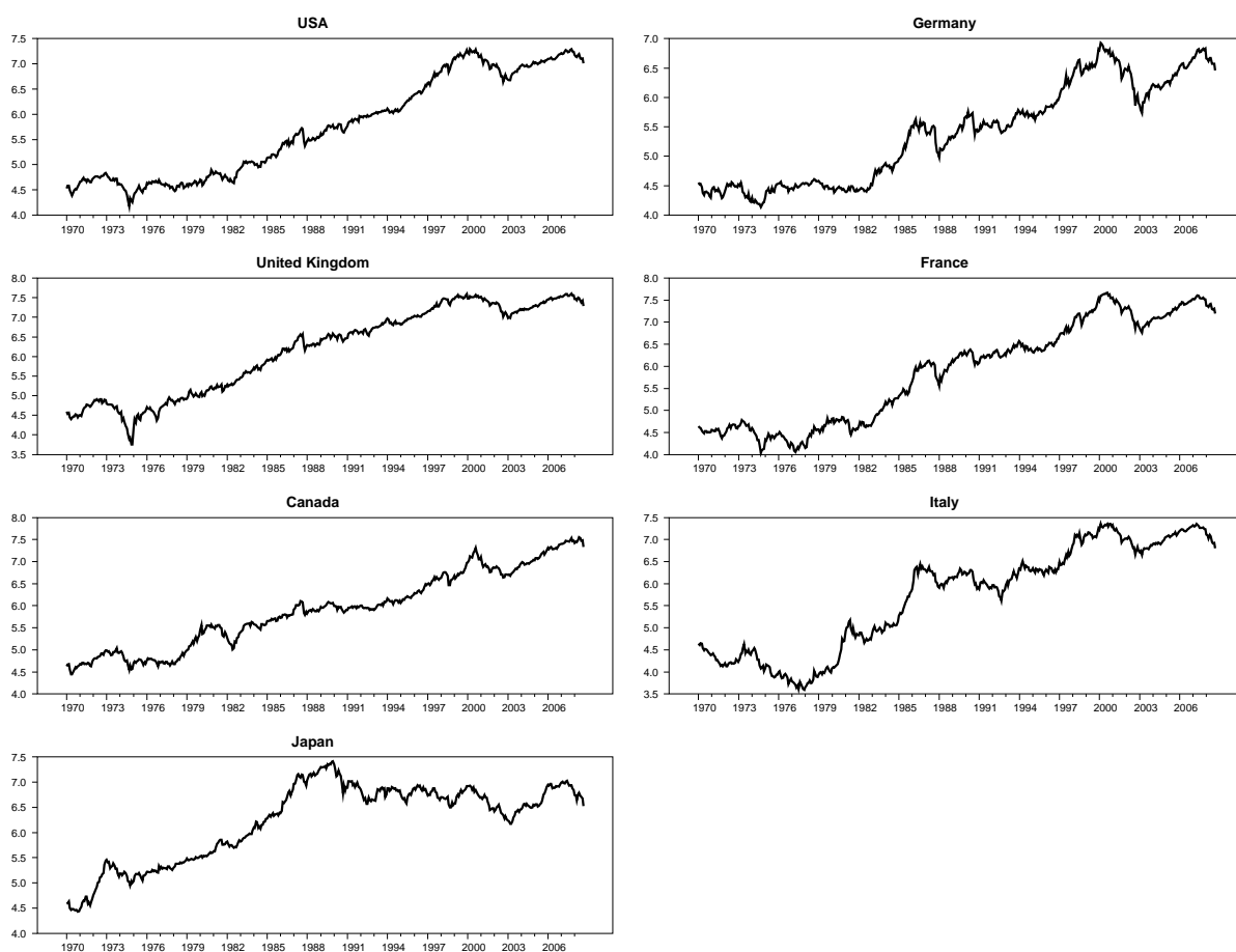
Figure 1: Log stock prices 1970/01-2008/10 (MSCI series are in the domestic currency)
