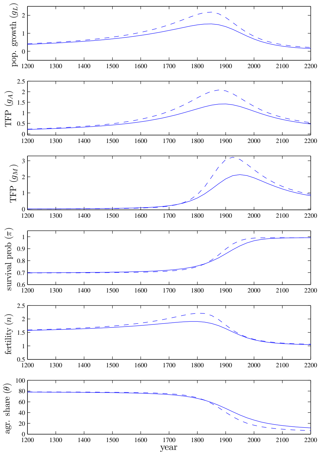
Figure 2: Long-Run Dynamics
