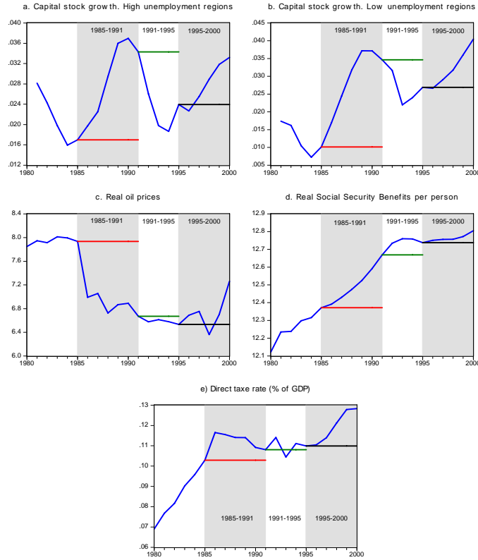
Figure 4. Exogenous variables in the empirical model
