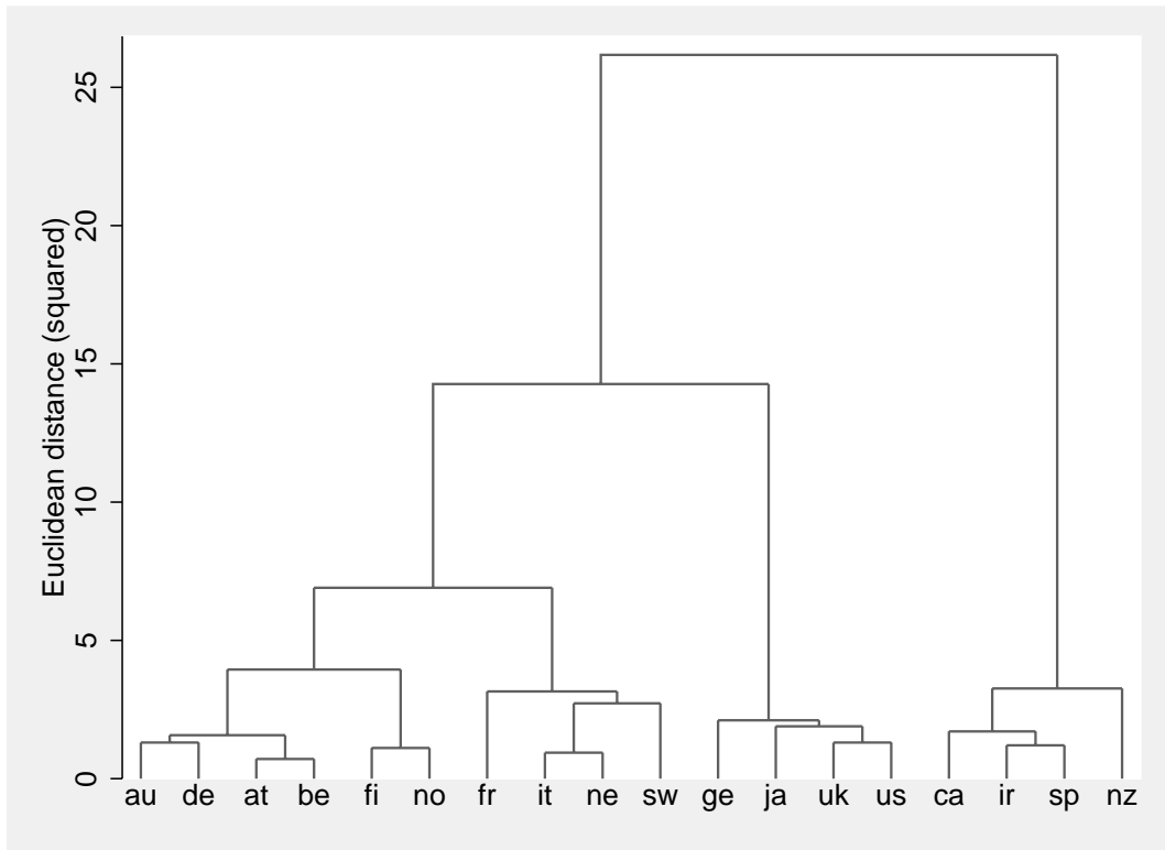
Figure 5. Cluster analysis
