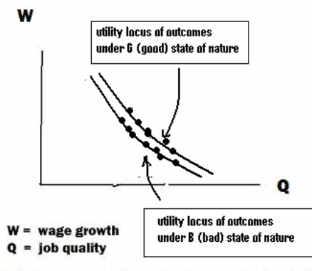
Fig. 2 - “squeezed” utilities allow identification (the graph displays the outcomes with many decision makers holding different payoffs)
