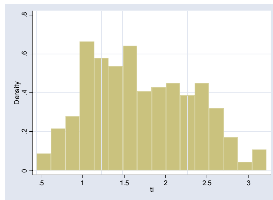
3.4 Interacted t-Statistics
