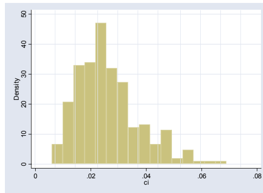
3.2 Interacted Coefficients
