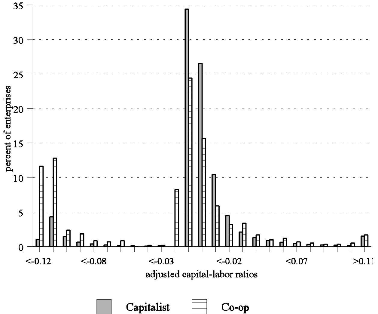
Frequency Distribution of Capital-Labor Ratios for Capitalist and Co-op Enterprises
