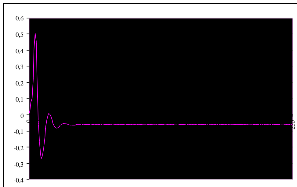
Figure 7: Cycles of the Real Growth Rate (Case 3)
