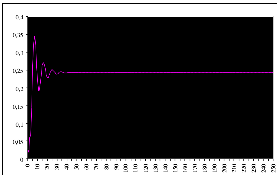
Figure 5: Cycles of the Real Growth Rate (Case 1)
