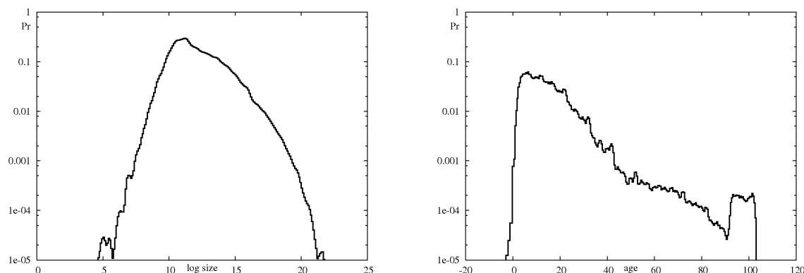
Figure 1: Kernel densities of the size distribution (log output in 2000; left) and age distribution (right), both plotted with a logarithmic y -axis. Kernel densities are computed for equispaced points using an Epanechnikov kernel (using the gbutils 5.1 software package).
