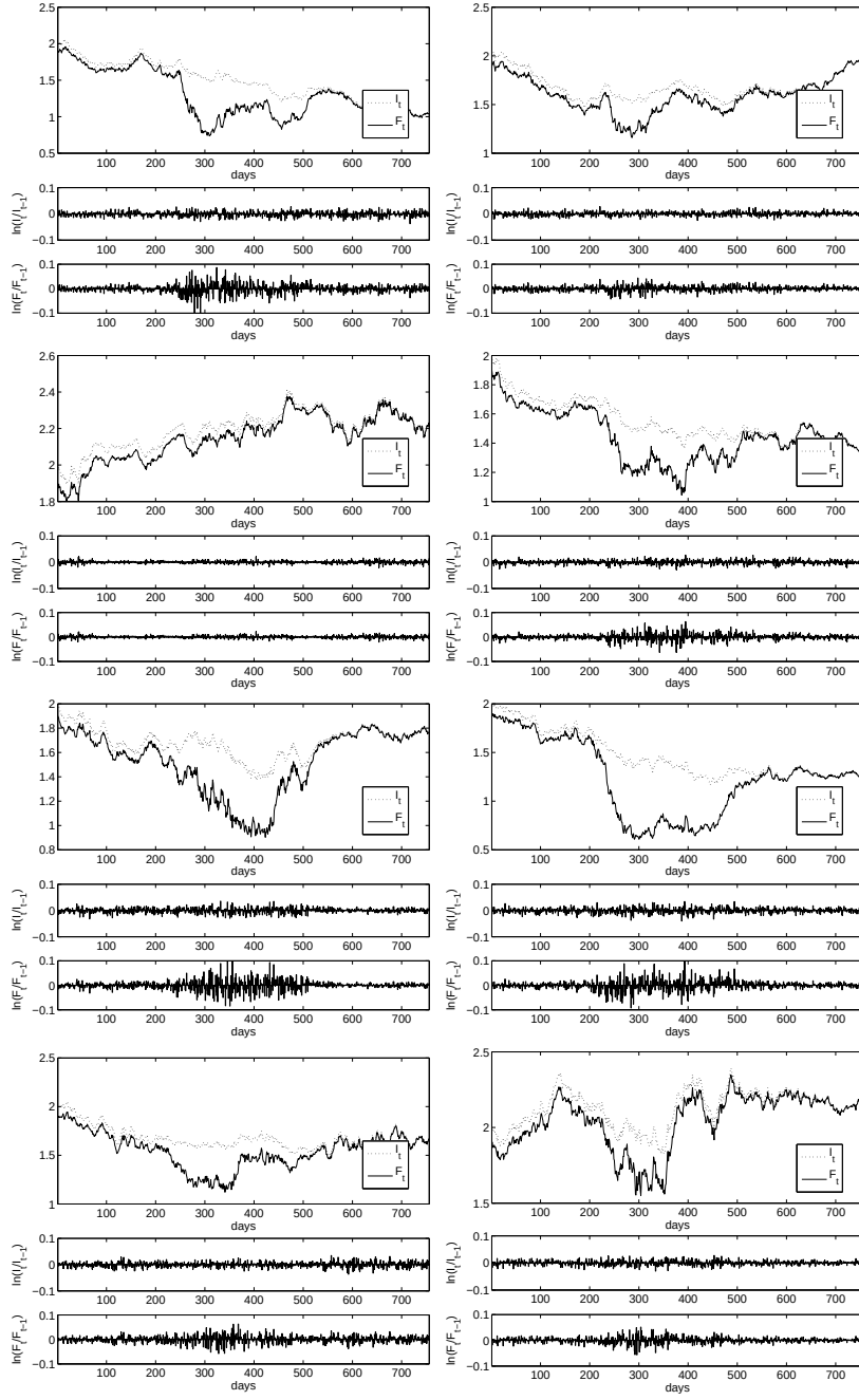
Fig. 3: Simulated time series for asset price F_t and information I_t for a time-dependent two-term pricing kernel ( N = 2 , \alpha_1 = 1 , \alpha_2(t) = 2.5[\tanh(10(t-1)) + \tanh(-10(t-2))] , \delta_1 = -1 , \delta_2 = -10 ). The ASPK switches smoothly from constant elasticity to declining elasticity and back. Logarithms of daily returns for F_t and I_t are shown below each graph. Time horizon is T - t = 3 years (756 business days) and other parameter values are as shown in Table 1 except \sigma_0 = \theta = 0.016641 .
