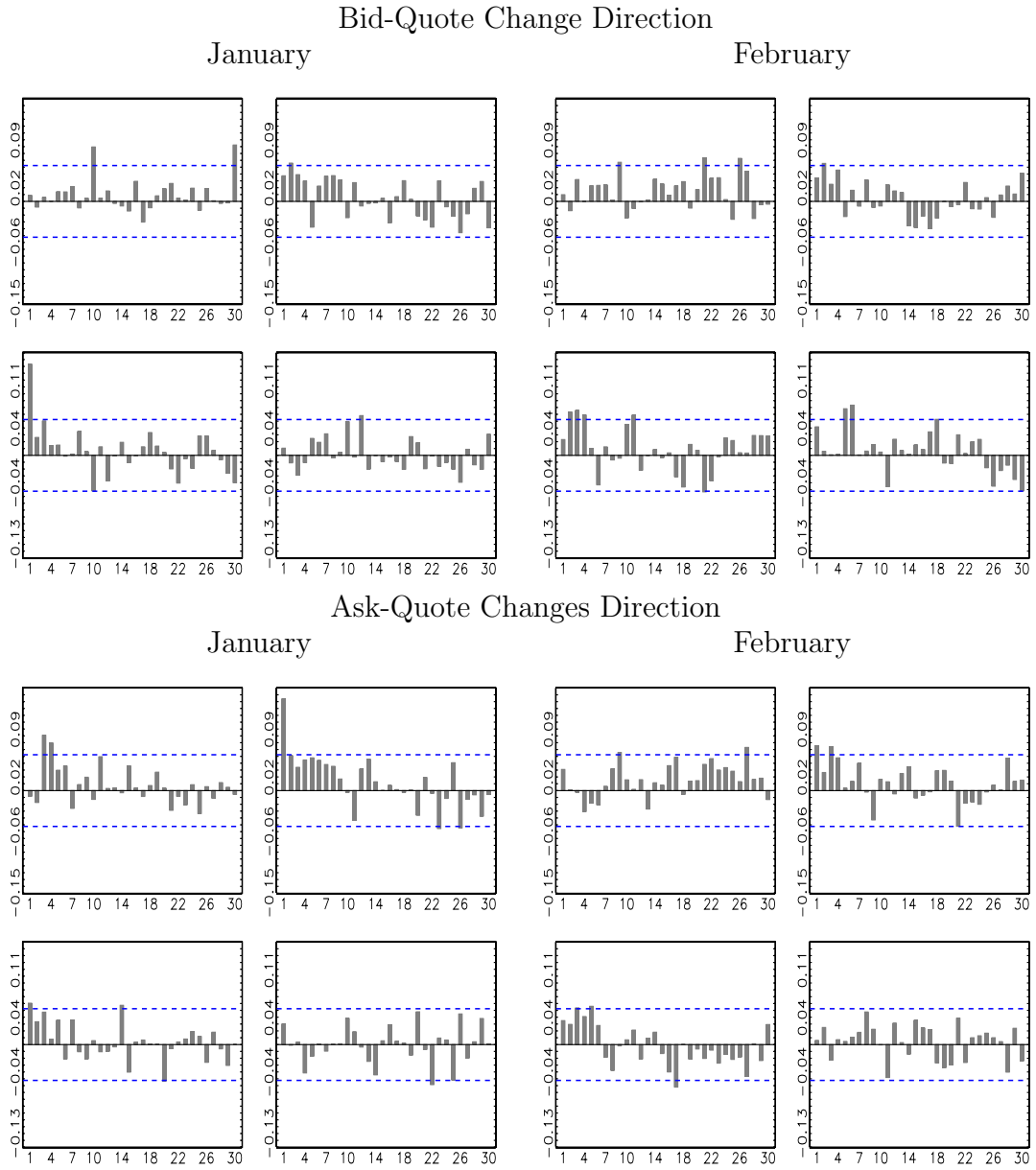
Figure 3: Multivariate-Autocorrelogram of the bid-quote change direction (upper panels) and ask-quote change direction (lower panels) in January (left panels) and February (right panels) for the BDK stock. The dashed lines denote asymptotic 95% confidence bounds.
