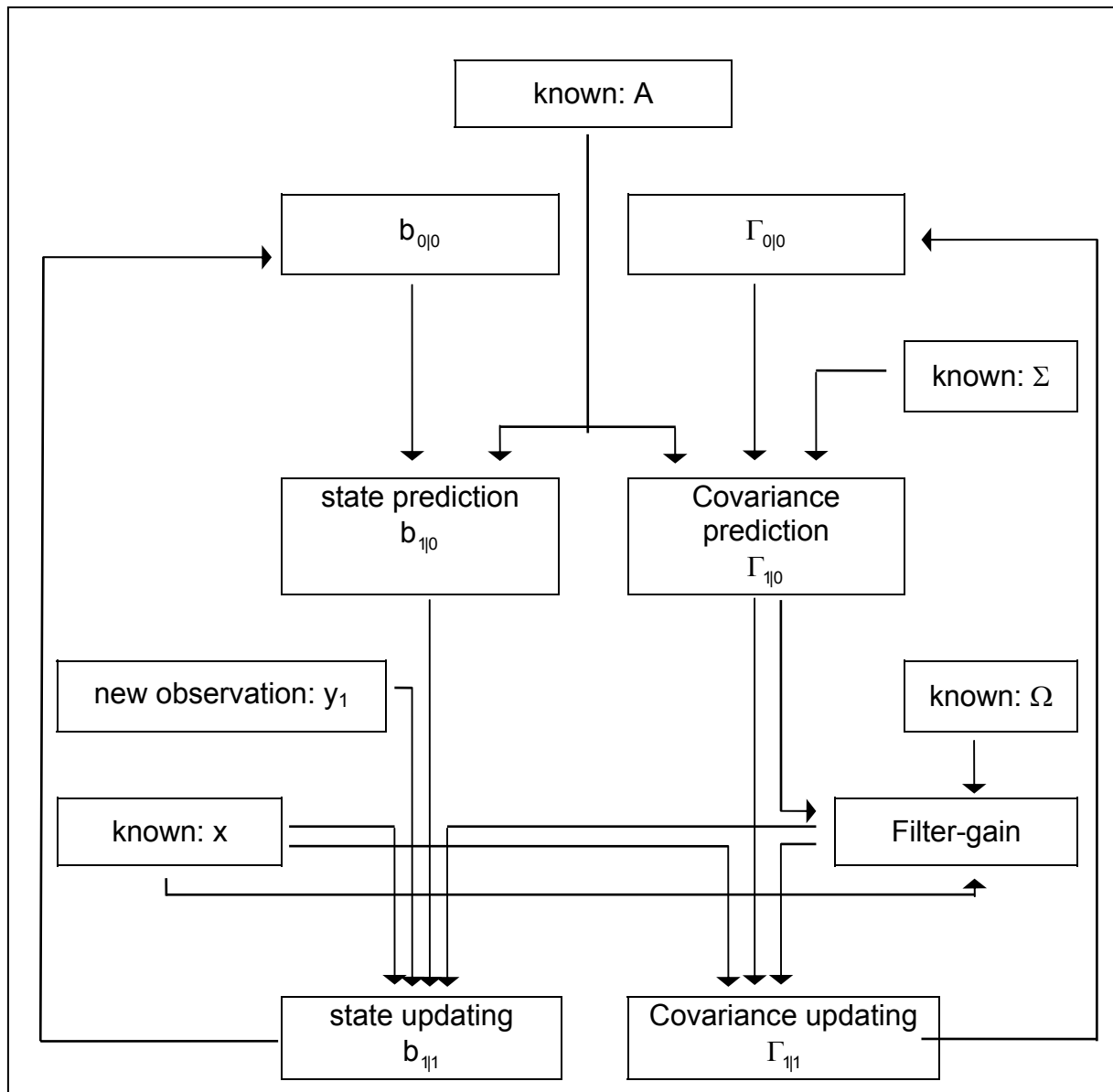
Fig. 2 Kalman-Filtering Algorithm
