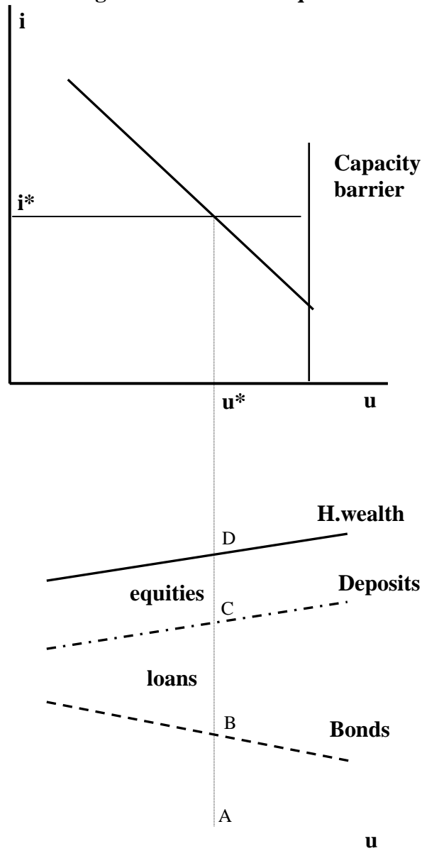
Figure 2. Short-Run Equilibrium
