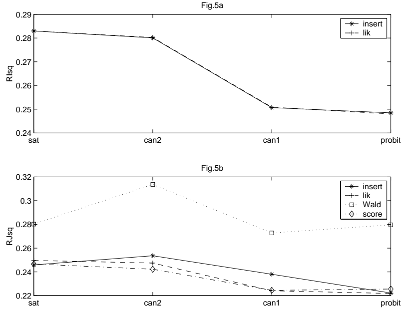
Figure 5: a) Estimates and estimates of approximations of R^2_{I,\pi_0} b) Estimates and estimates of approximations of R^2_{J,\pi_0}
