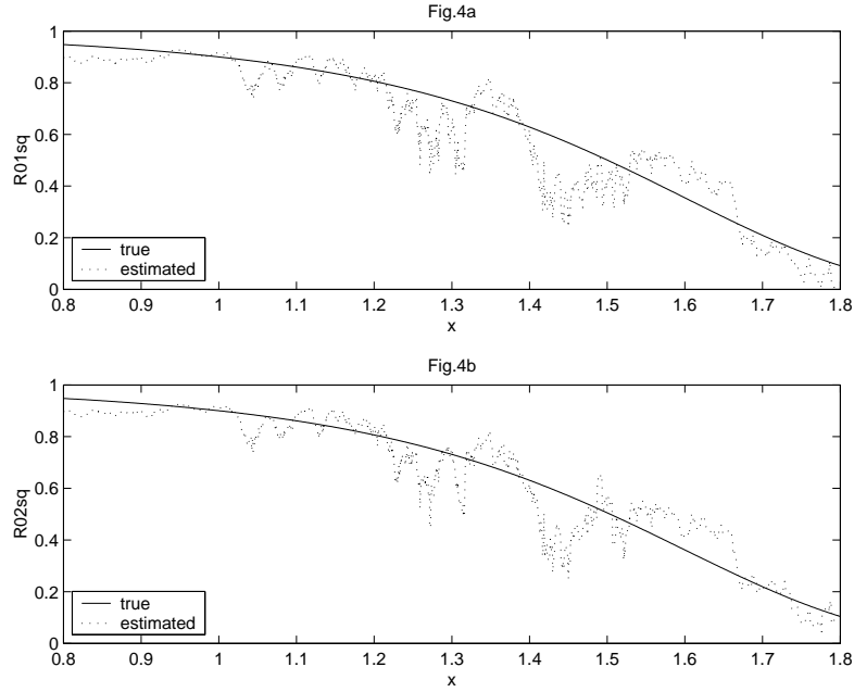
Figure 4: a) true and estimated correlation curve \rho^2(x) = \text{determination curve } R_{J_{01}}^2(x) with estimate based on K = 300 b) determination curve R_{J_{02}}^2(x) with estimate based on K = 300
