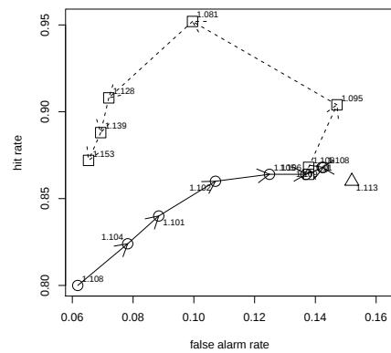
Figure 5: Pseudo-ROC curves for the identification of influential and non-influential covariates with metric response data for PartBoostR (circles) and elastic net (squares) with varying penalty parameters (and the optimal number of steps) and for the Lasso (triangle). Arrows indicate increasing penalty parameters. The numbers give the mean squared error of prediction for the respective estimates.
