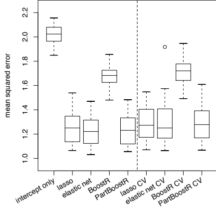
Figure 4: Mean squared error for continuous response data with varying number of predictors p and correlation \rho_b for the linear model including only an intercept term, elastic net, the Lasso BoostR and PartBoostR with tuning parameters selected for optimal performance or by cross-validation (CV).
