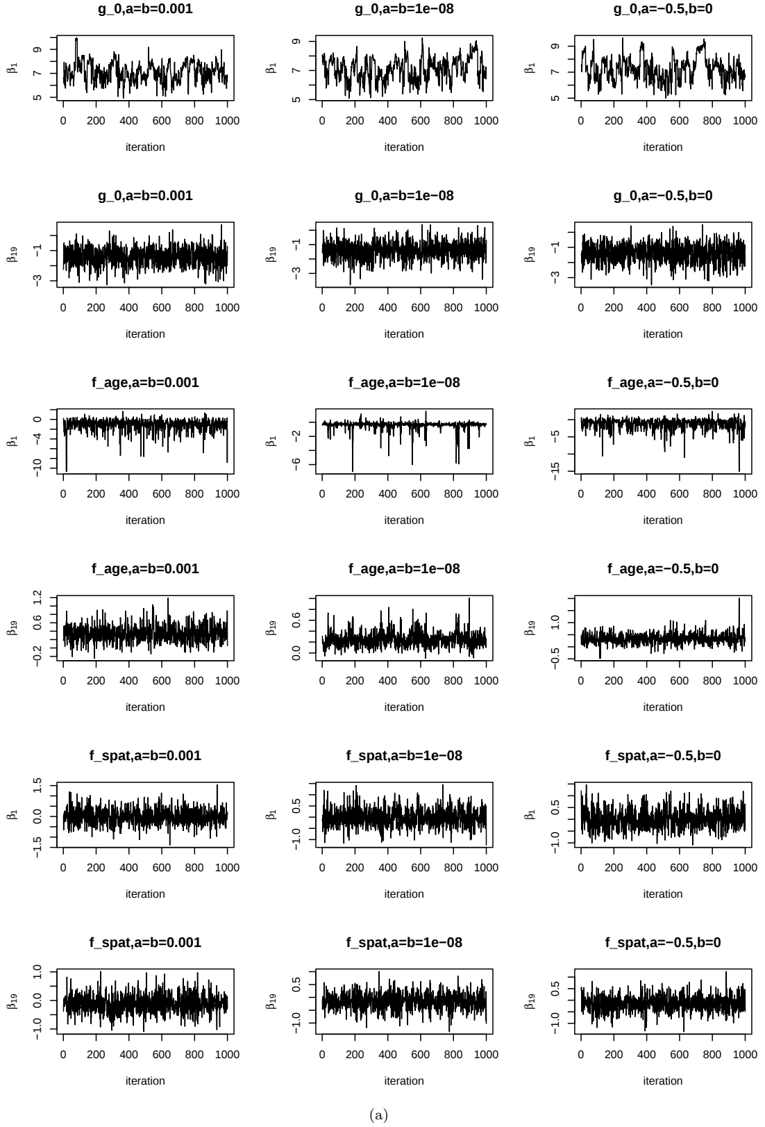
Figure 6: Selected sampling paths for parameters \beta_{j,1} and \beta_{j,19} , j = 0, age, spat and different choices for the parameters a and b of the IG(a; b) hyperpriors.
