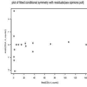
Figure A.1: Fitted symmetry with Residual for sex opinions poll Figure A.2: Fitted conditional symmetry with Residual for sex opinions poll
