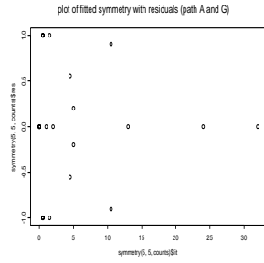
Figure A.3: Fitted symmetry with Residual for path A and G Figure A.4: fitted Conditional Symmetry with residuals for path A and G
