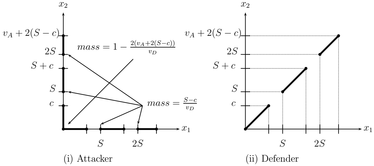
Figure 1: Supports of case (a) equilibrium joint distributions with \lfloor \frac{v_A}{c} \rfloor = 2 and n = 2 .
