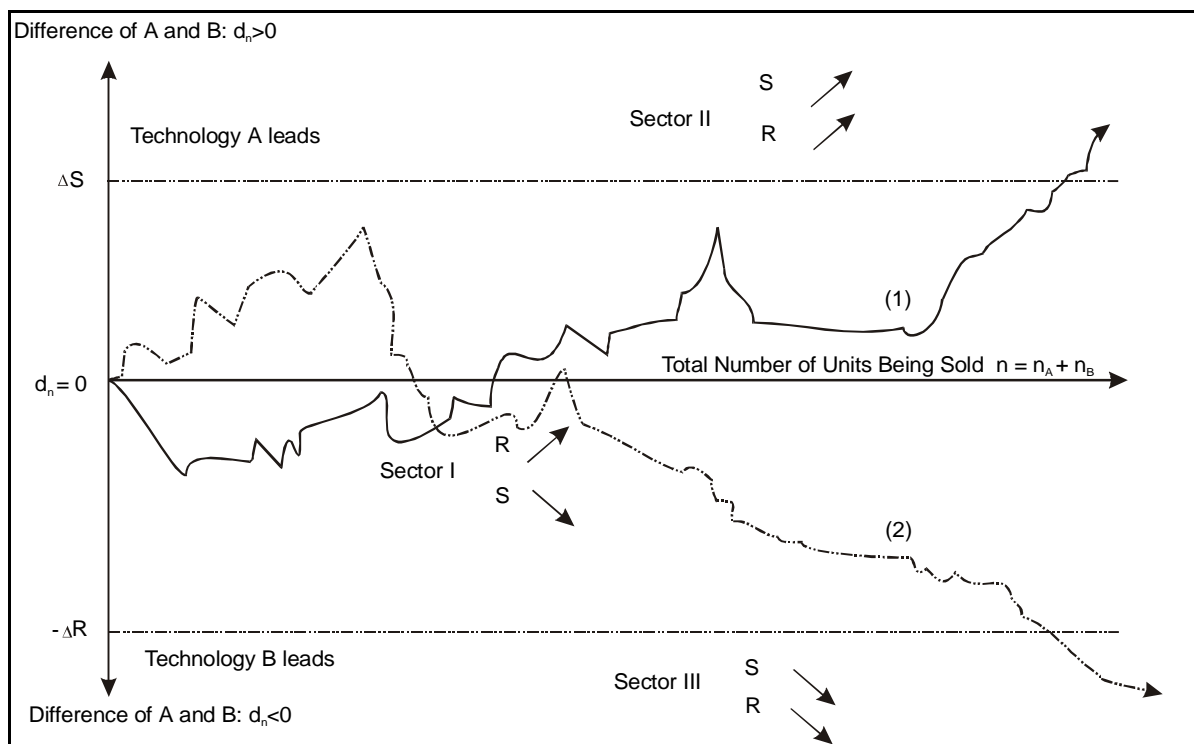
Fig. 5: Allocation processes under positive feedback. Source: ARTHUR (1997b), p. 23 and own drawing (2001).
