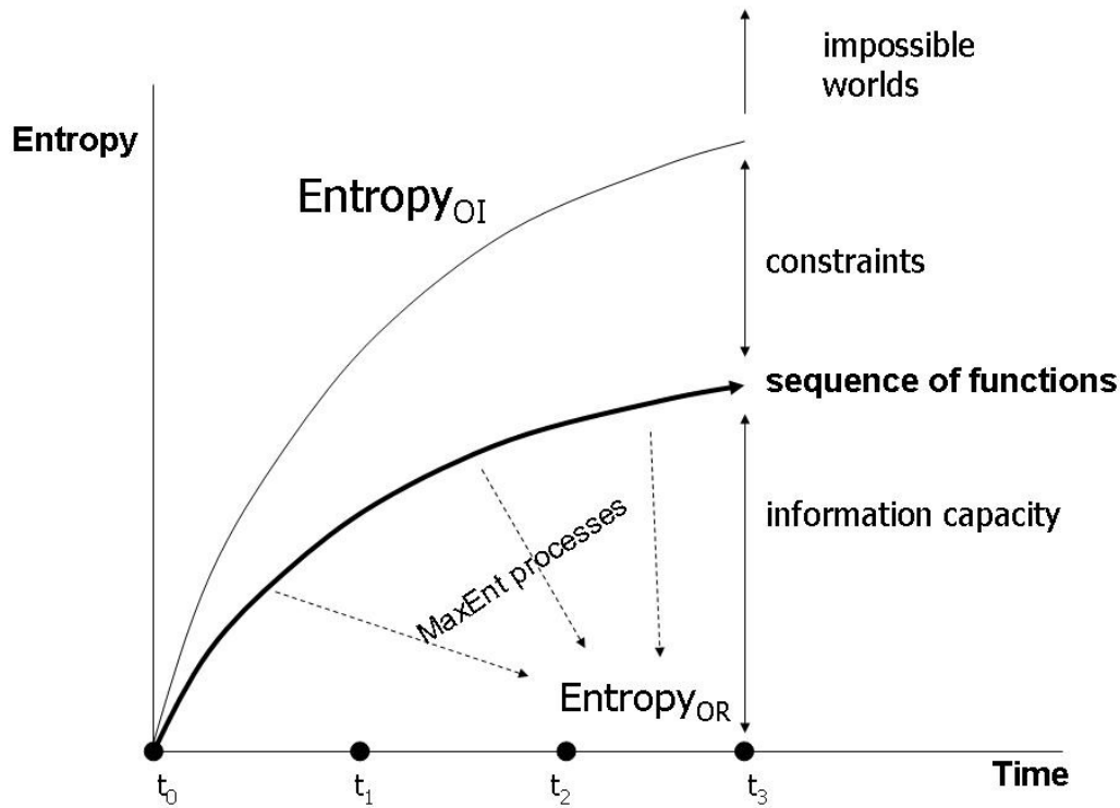
Figure 7: Evolution of entropies
