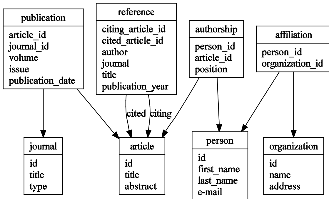
Figure 2: Diagram of the basic relational schema
