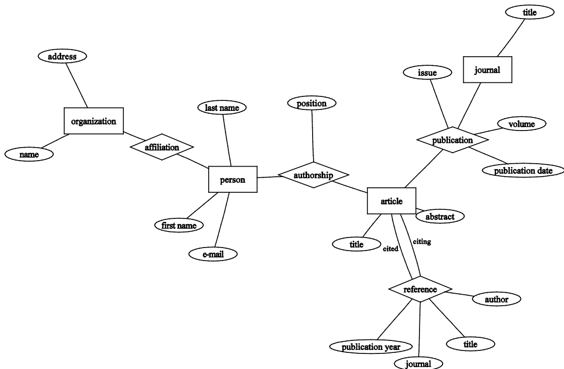
Figure 1: Basic ER diagram
