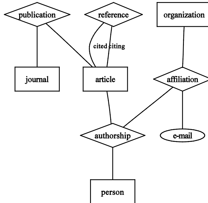
Figure 3: ER diagram with adjusted affiliation relationship
