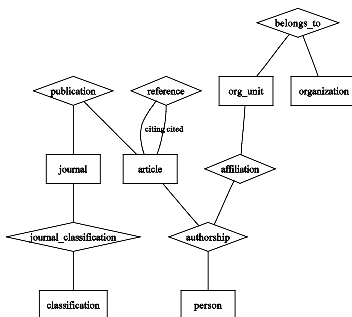
Figure 4: Final ER diagram: organizational unit and classification added
