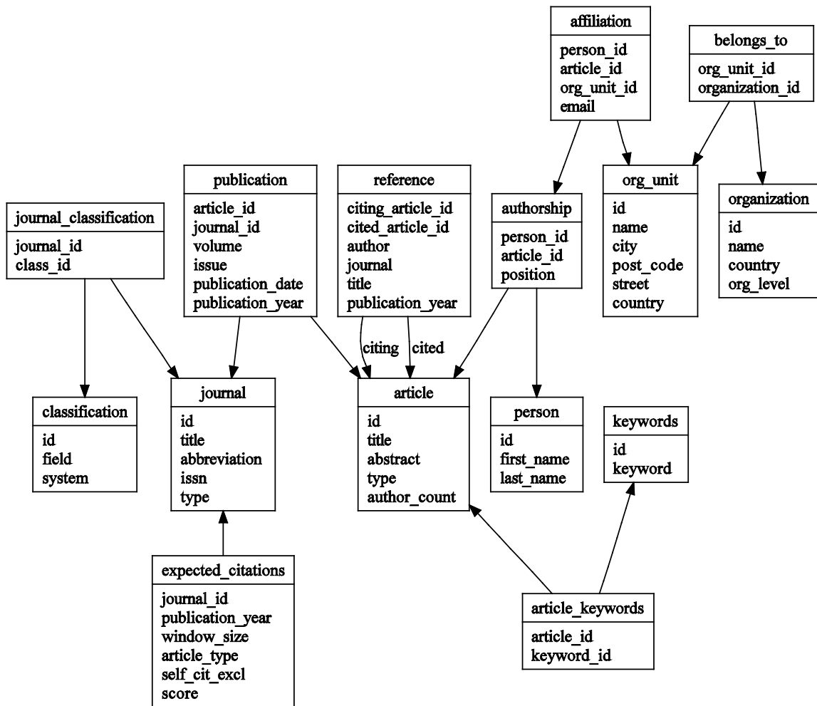
Figure 5: Final relational database schema
