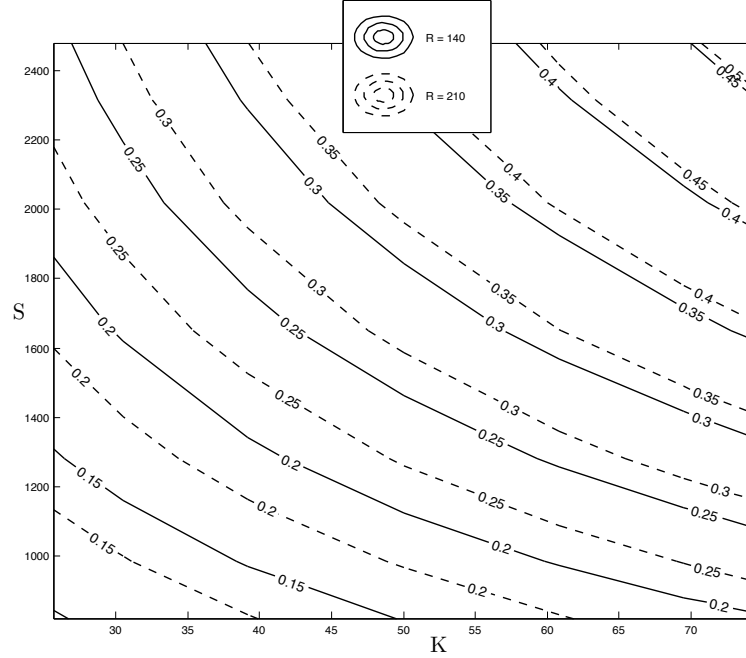
Figure 2: Optimal mitigation for \sigma = 0.05 and different levels of R
